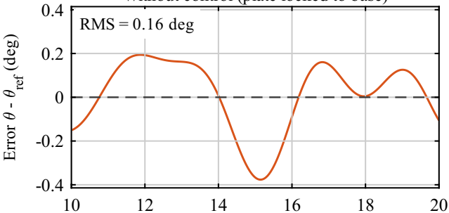
Without control (plate locked to base)
